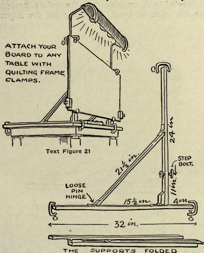
Construction of Plain Supports and Stationary Board Reproduced by courtesy of the Federal Schools, Inc.
